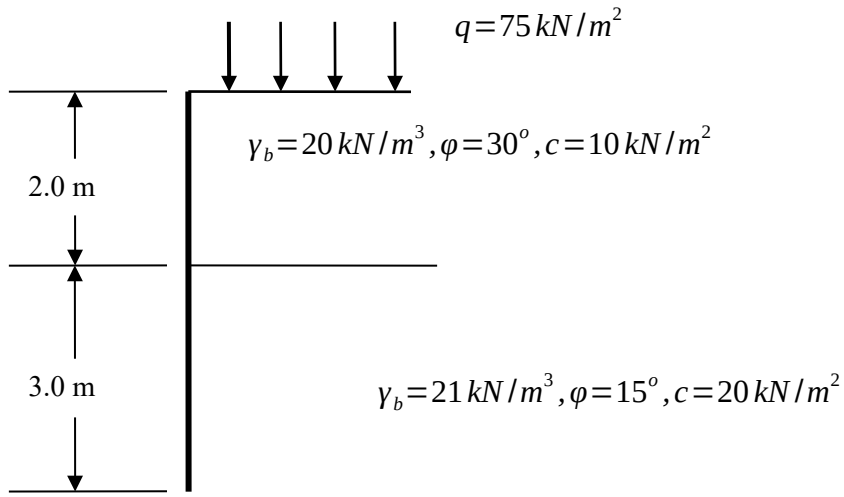
Fig. 1.1: Retaining wall
