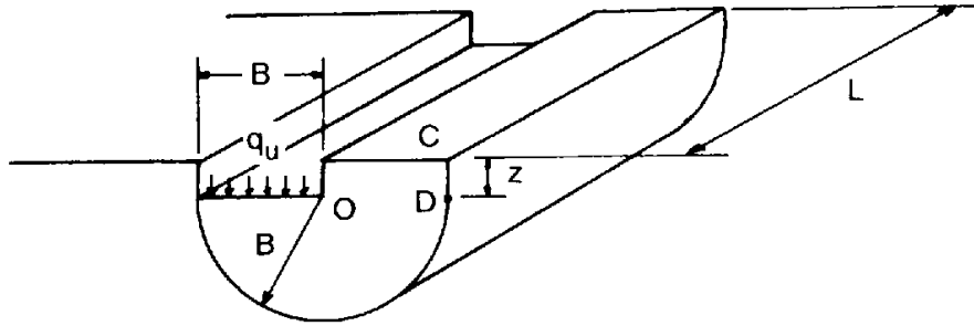
Fig. 3.1: Slip circle failure mechanism
