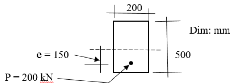
Fig. 4.1: Pre-stressed beam
