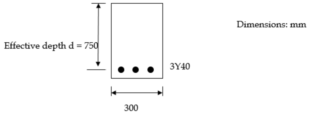
Figure 1.1: Rectangular Reinforced Concrete beam
