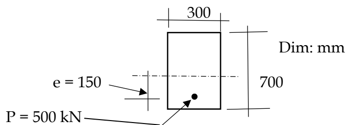
Fig. 4.1: Pre-stressed beam
