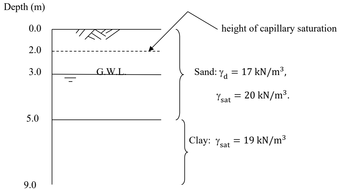
Figure 4.1: Details of a borehole log
