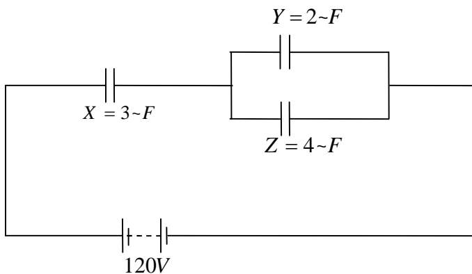
Figure 2 : Capacitors
